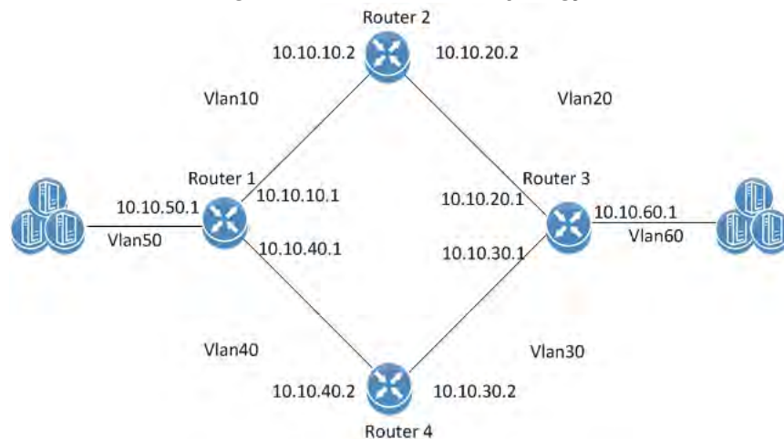
Figure 36: OSPF Basic Topology
