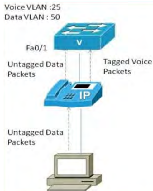
Figure 20: Tagging Voice Packets with a Different VLAN ID
