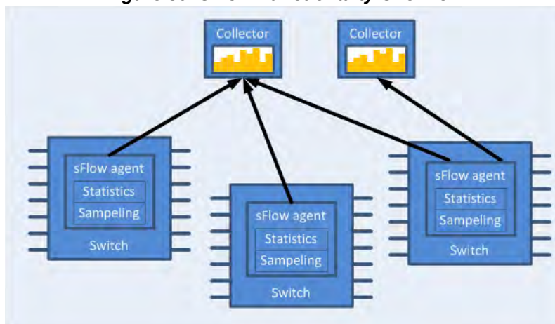
Figure 30: sFlow Functionality Overview
