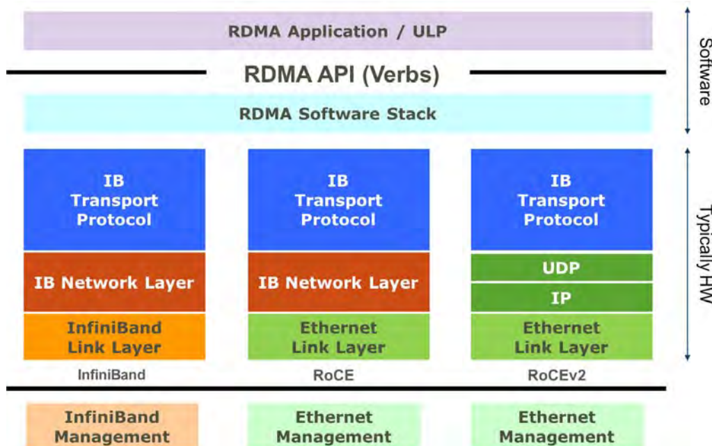
Figure 32: RoCEv2 Protocol Stack
