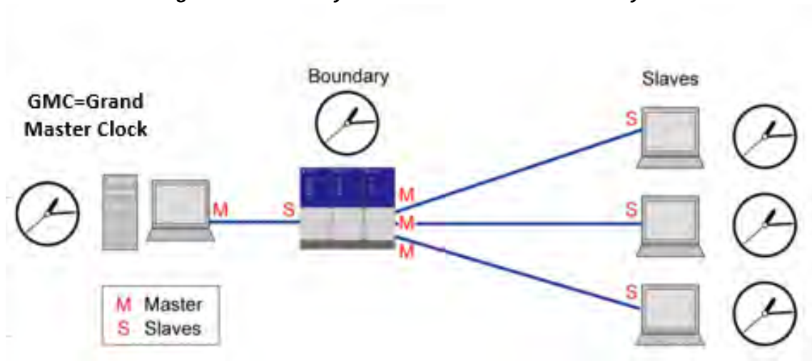
Figure 13: Boundary Clock Master/Slave functionality
