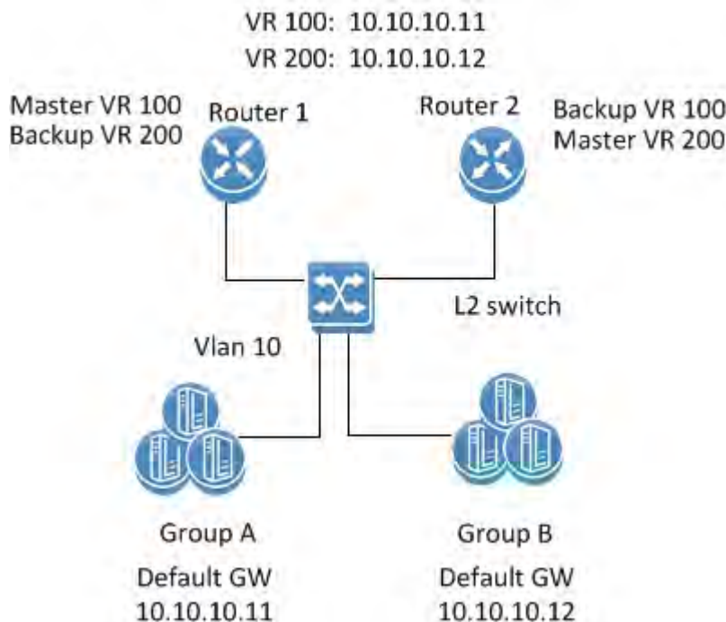
Figure 38: Common VRRP Configuration with Load Balancing
