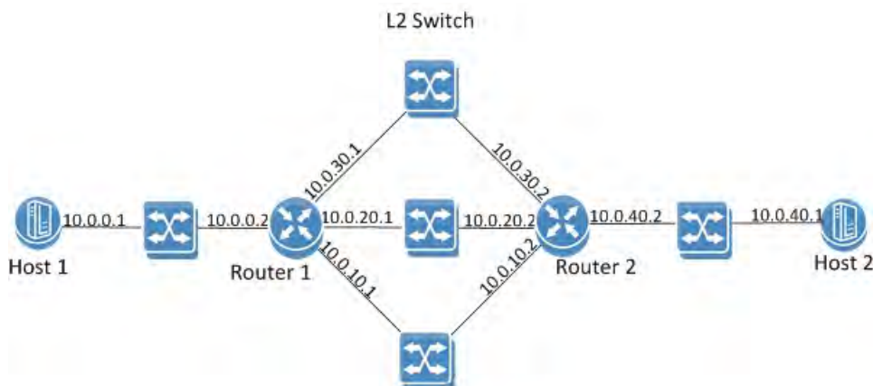
Figure 34: ECMP
