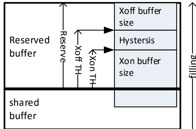
Figure 33: Xon/Xoff Configuration
