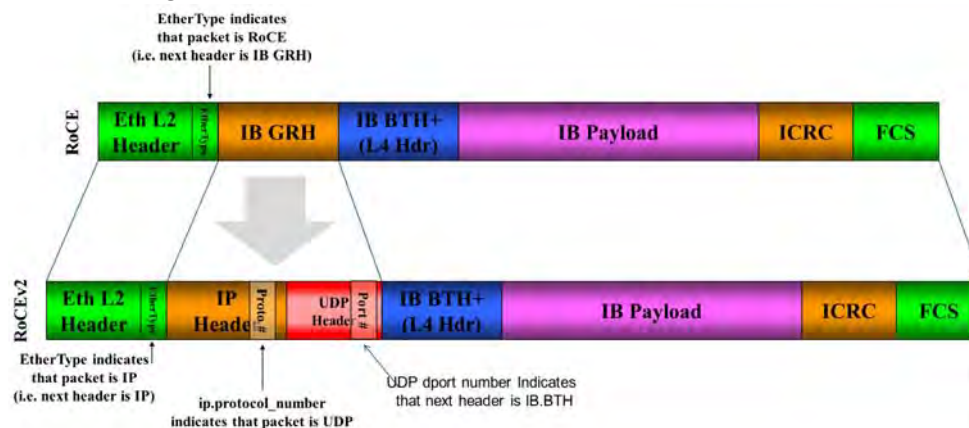
Figure 31: RoCEv2 and RoCE Frame Format Differences
