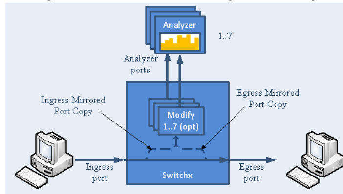
Figure 26: Overview of Mirroring Functionality
