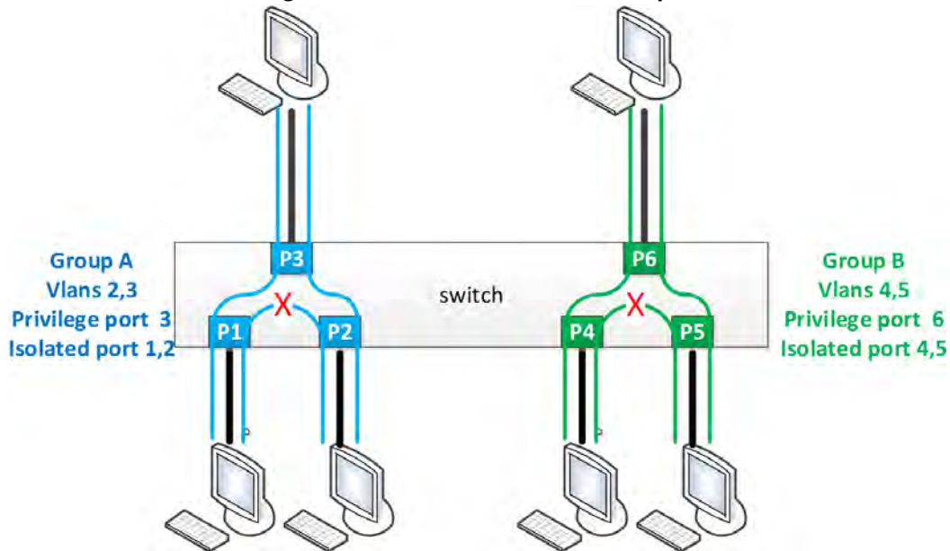
Figure 17: Interface Isolation Example
