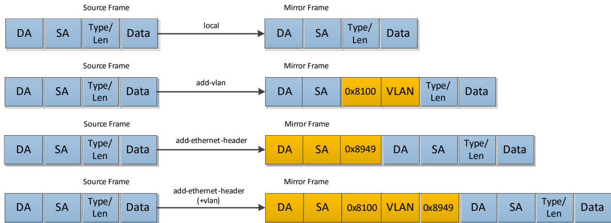
Figure 28: Header Format Options
