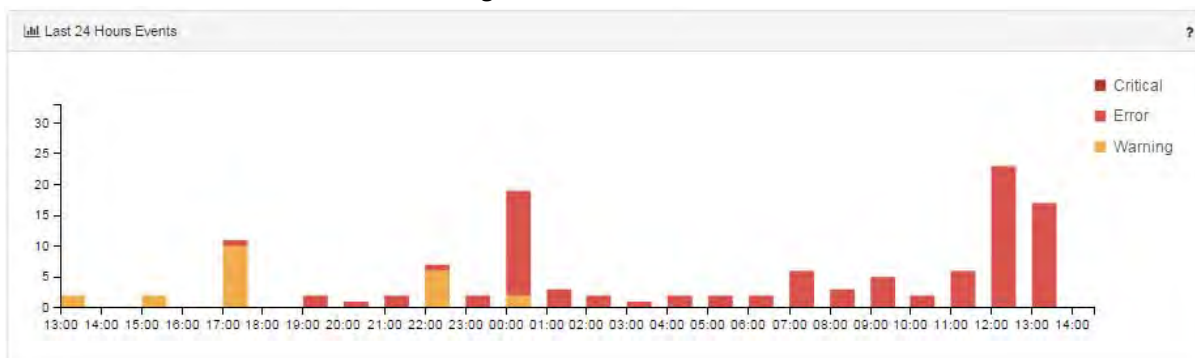
Figure 42: 24-Hour View
