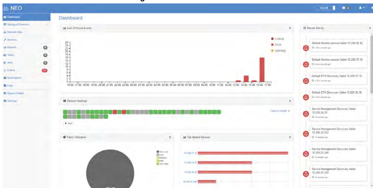
Figure 41: Fabric Dashboard
