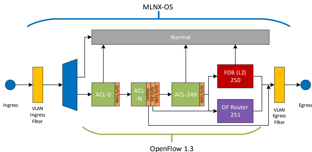
Figure 24: MLNX-OS and OpenFlow Pipeline
